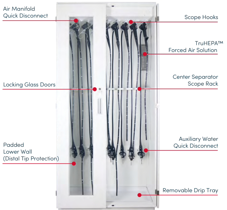
SAS-9P-HA, SAS-18P-HA Full Width TruAir Scope Drying Cabinet
