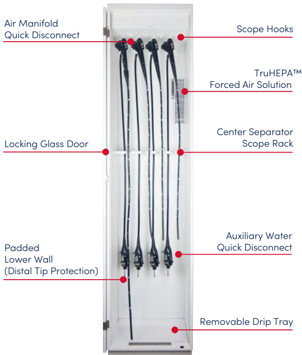
SAS-4P-HA, SAS-8P-HA Half Width TruAir Scope Drying Cabinet
